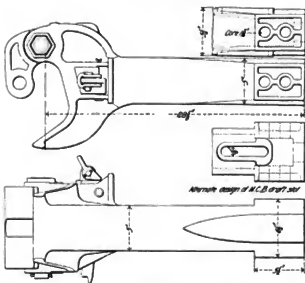
Figs. 3999-4002. Washburn Coupler, Type A. Washburn Coupler Co.
